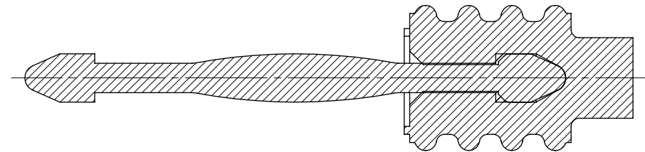
SECTION B-B
