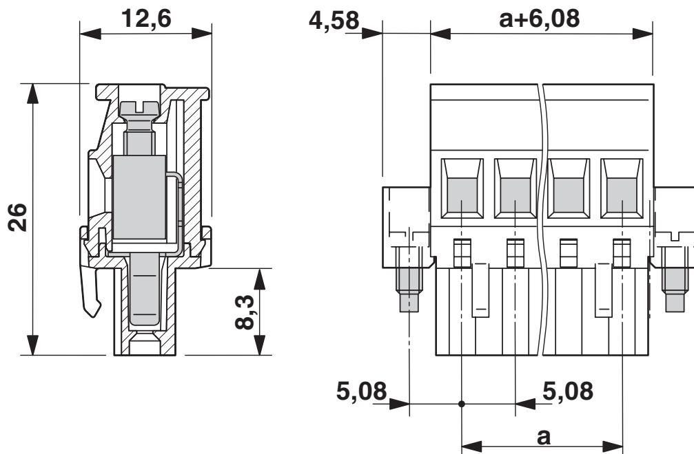
Dimensional drawing
